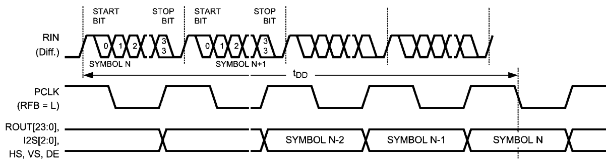
FIGURE 4. Delay - Latency
