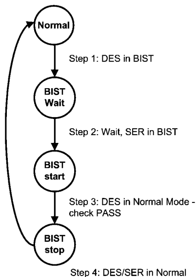
FIGURE 17. BIST Mode Flow Diagram
