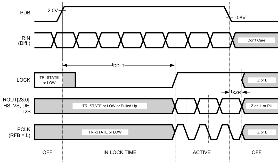
FIGURE 5. PLL Lock Times and PDB TRI-STATE Delay
