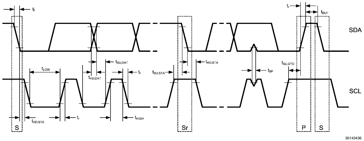
FIGURE 9. Serial Control Bus Timing Diagram
