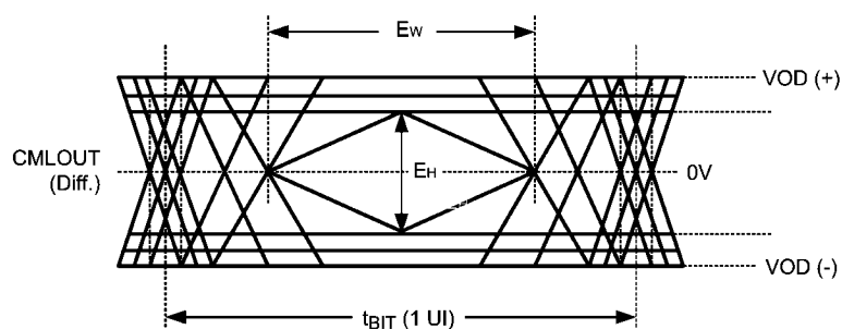
FIGURE 2. CML Output Driver
